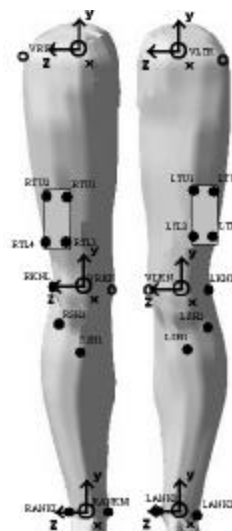
Figure 1: Biomechanical model, lower body used to derive kinematics of hip and knee. Local coordinate systems shown.
